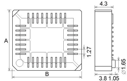
PLCC - 44 NTT-5 SMD
